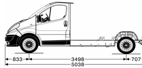
Vivaro Floor Cab
