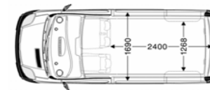
Vivaro Double Cab L1 H1
