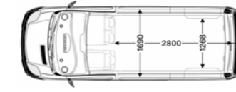
Vivaro Double Cab L2 H1
